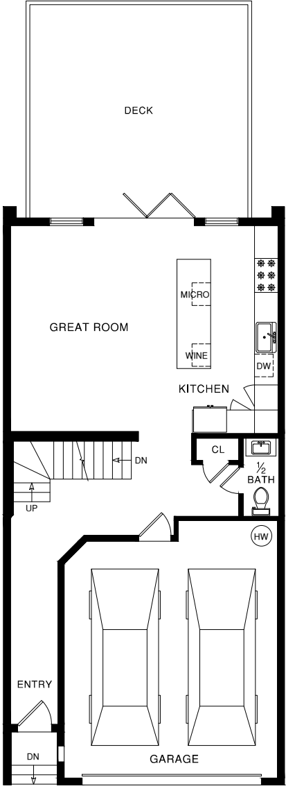
MAIN LEVEL
